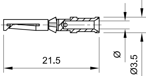
Female contact
