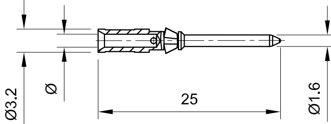
Male contact
